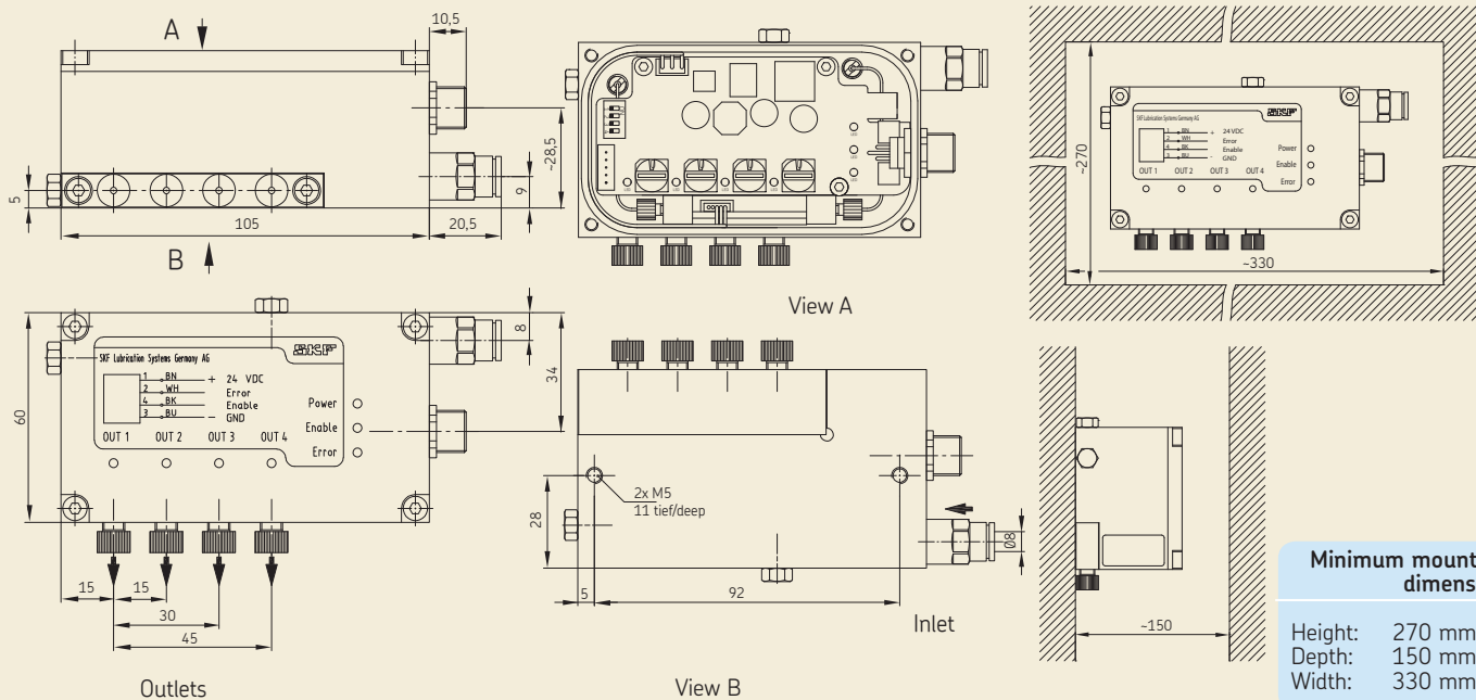
Assembly drawing of the MDU micro-metering unit, Fig. 5
