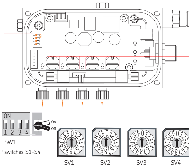
Rotary switches SV1 to SV4 = lubrication point 1 to lubrication point 4
