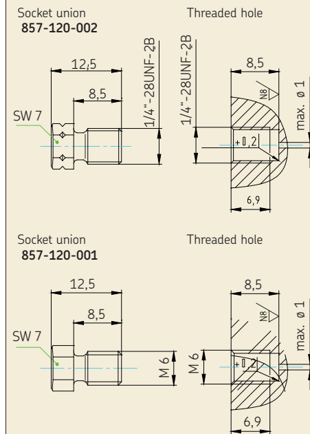
Connection versions on the spindle side, Fig. 1
