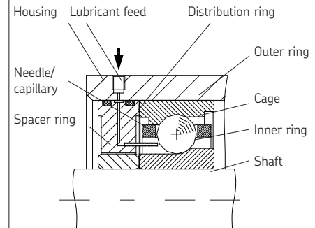
Lubricant feeding for vertical and horizontal mounting position and rotating inner ring, Fig. 2
