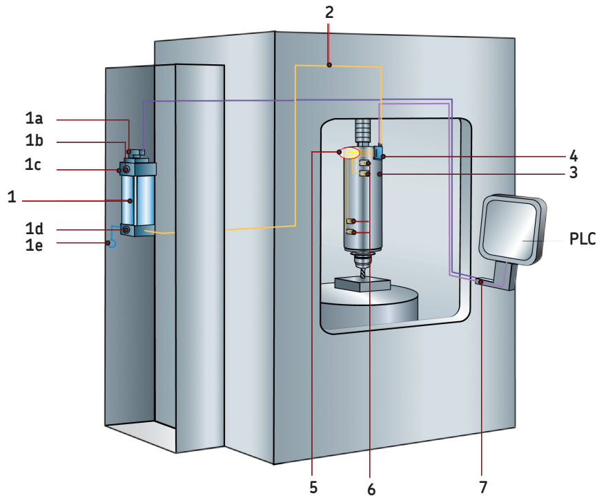
Application example of the microdosage system on a machine tool
