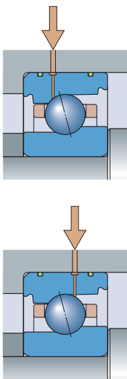
Lubricant feeding via outer ring, Fig. 3
